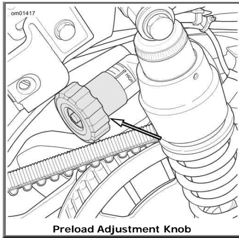
Manual Suspension Preload Table: Models with Tour-Pak
